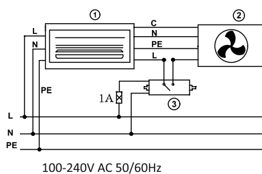
(2) Strong electric control connection (current <3A)
